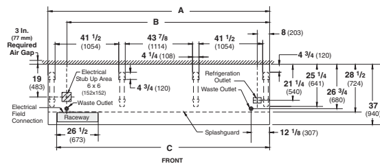
D5NX-LE, D5NX-LEP Plan View
